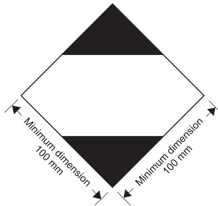
Figure 3.4.1: Mark for packages containing limited quantities
